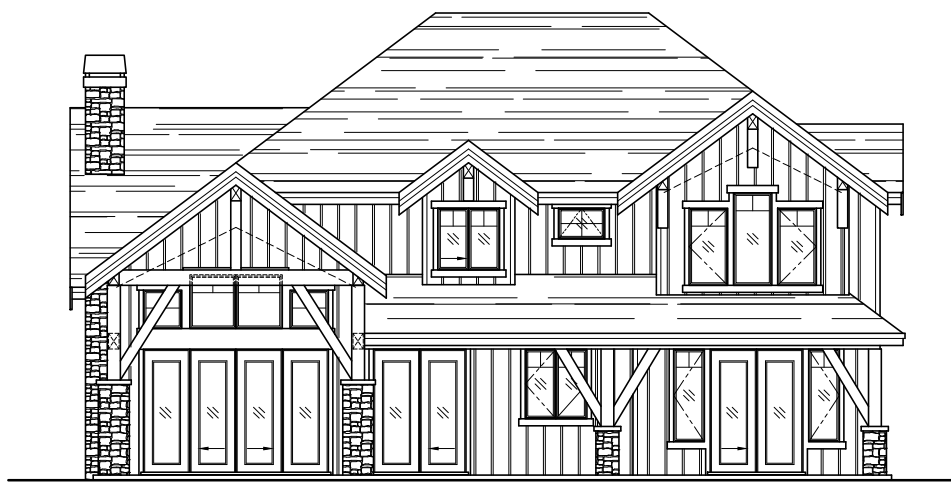
REAR ELEVATION
