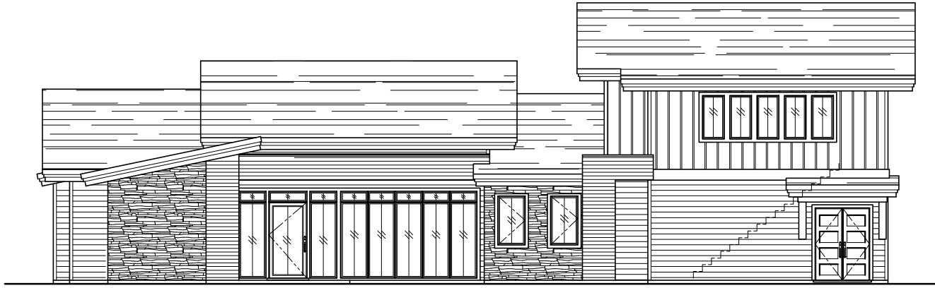
FRONT ELEVATION SEE GENERAL NOTES SCALE: 1/4" = 1'-0"
