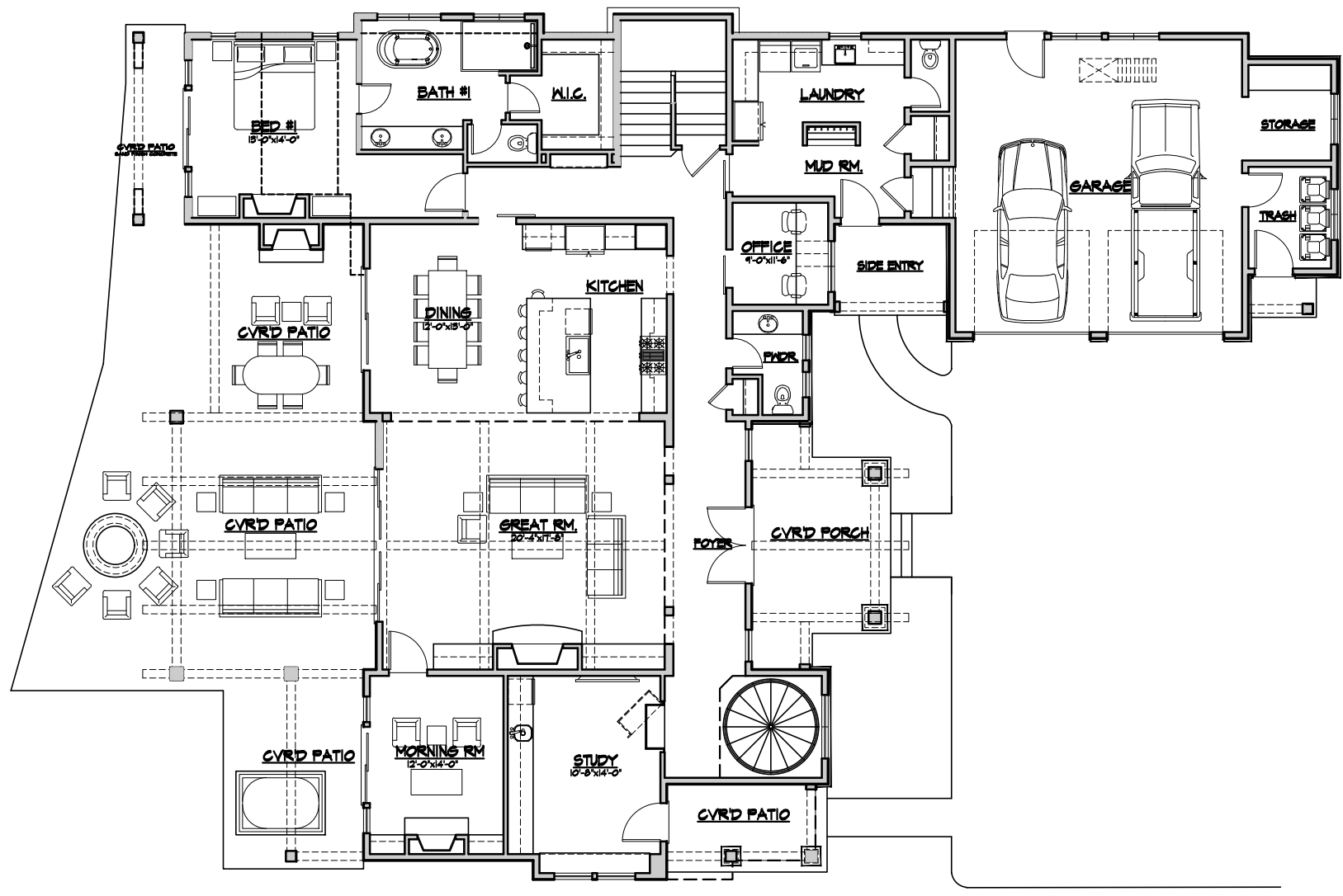
MAIN FLOOR PLAN
